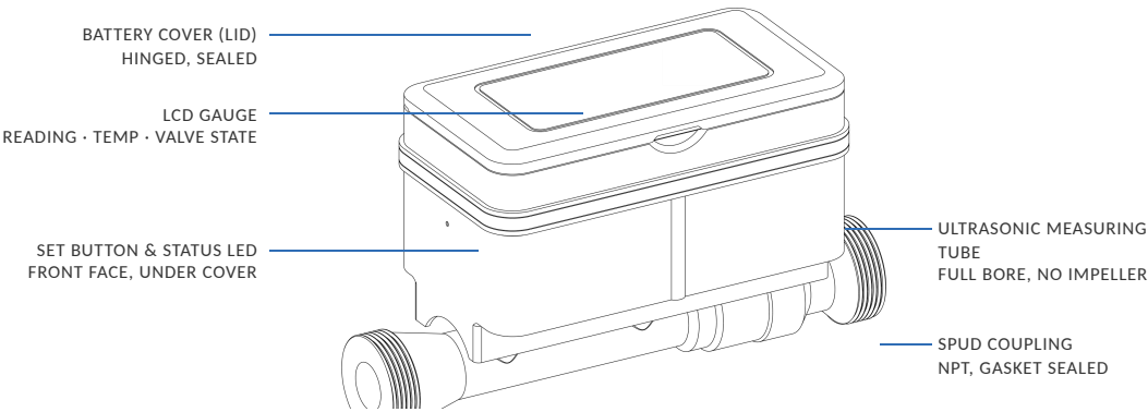
FIG. 01 • SHA-1000 — ISOMETRIC VIEW, DN20 SHOWN
