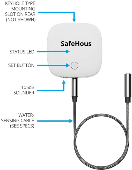
FIG. 01 • WS-1000 – ANNOTATED FRONT VIEW WITH 4.2 FT CABLE SENSOR
