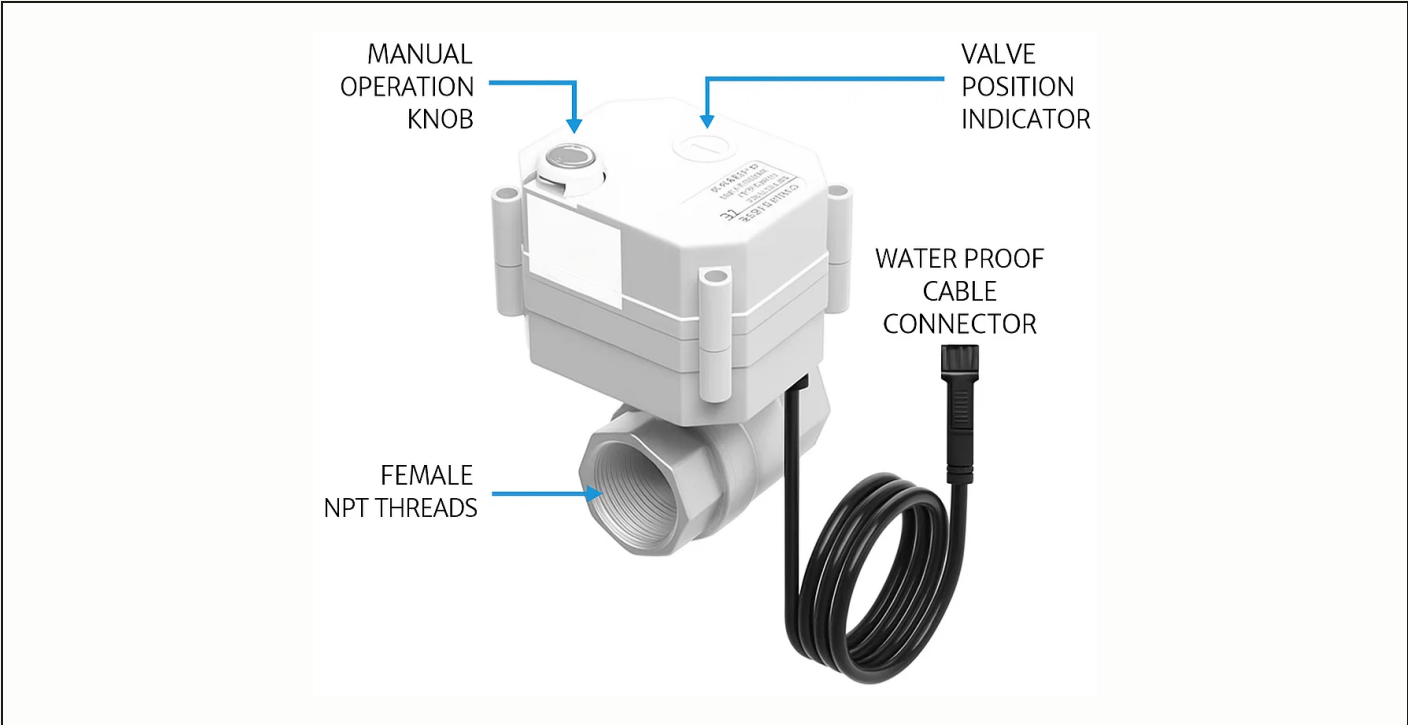
FIG. 01 • ASV-1000 – ANNOTATED MOTORIZED BALL VALVE WITH WATERPROOF CABLE CONNECTOR
